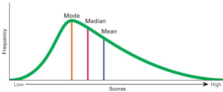
(a) Right-skewed distribution
