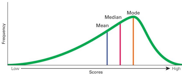
(b) Left-skewed distribution
